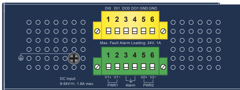
Figure 2-2: IVR-300/IVR-300W Upper Panel
