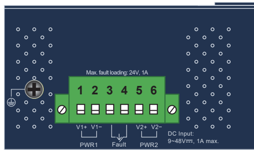
Figure 2-1: IVR-100 Upper Panel
