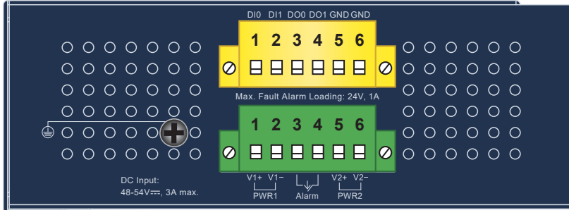
Figure 2-3: IVR-300FP Upper Panel
