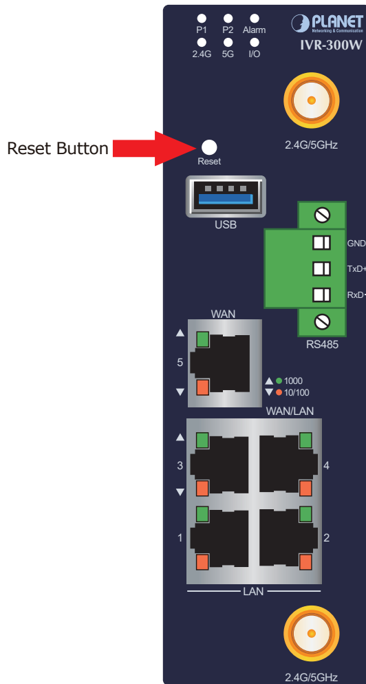
Figure 5-1: Reset Button of IVR-300 Series
