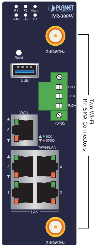
Figure 2-5: IVR-300W Front Panel
