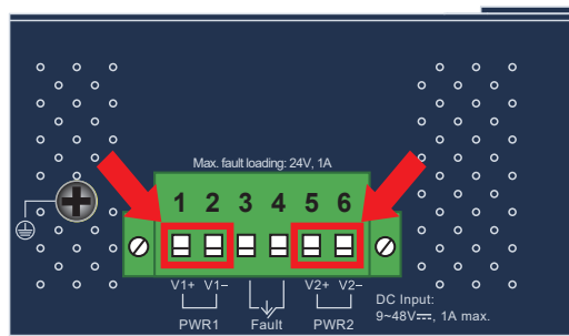
Figure 2-4: Power 1 and Power 2
